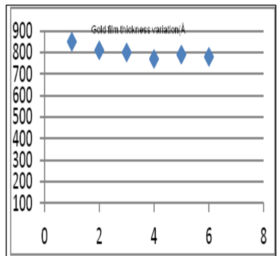
Fig 12: Measurement of Gold Film Thickness at 6 Points by Dektak
